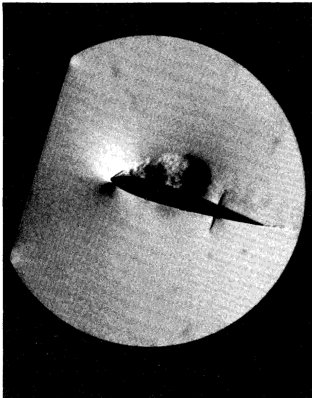
Fig. 4 Multiple vortices on a pitching airfoil: M = 0.25 , \alpha^+ = 0.025 , \alpha = 16.5 deg.
