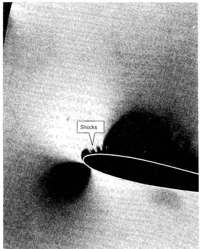
Fig. 5 Schlieren photographs of multiple shocks on a rapidly pitching airfoil: M = 0.45 , \alpha^+ = 0.0313 , \alpha = 12.6 deg.
