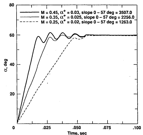
Fig. 1 Time history of pitching airfoil.
